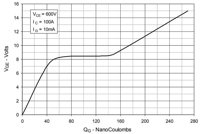
Fig. 8. Gate Charge
