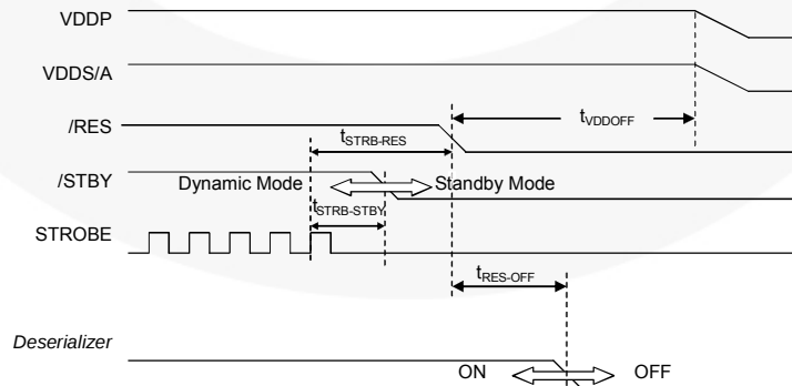
Figure 19. Power-Down Timing
