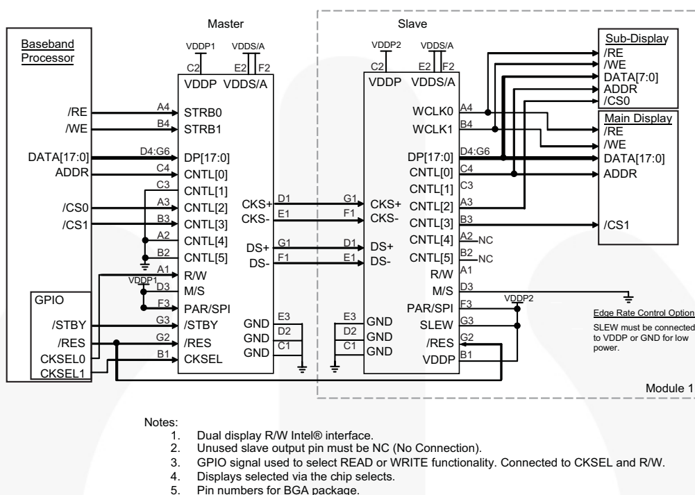
Figure 10. Dual R/W x86-Style Microcontroller Display Interface
