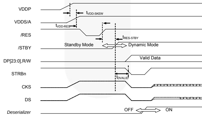
Figure 18. Power-Up Timing
