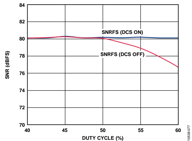
Figure 68. SNR vs. DCS On/Off, V_{REF} = 1.3\text{ V}
