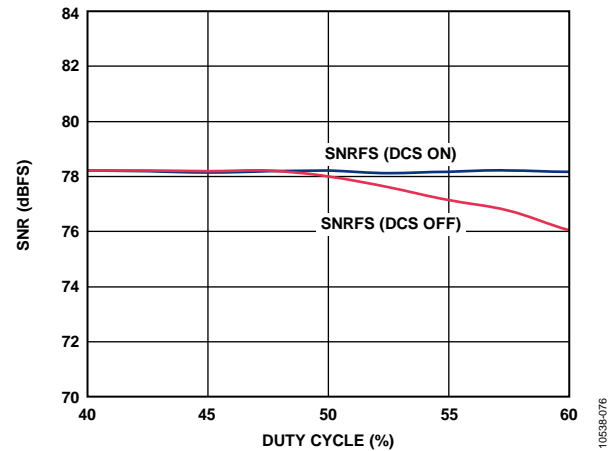
Figure 67. SNR vs. DCS On/Off, V_{REF} = 1.0\text{ V}
