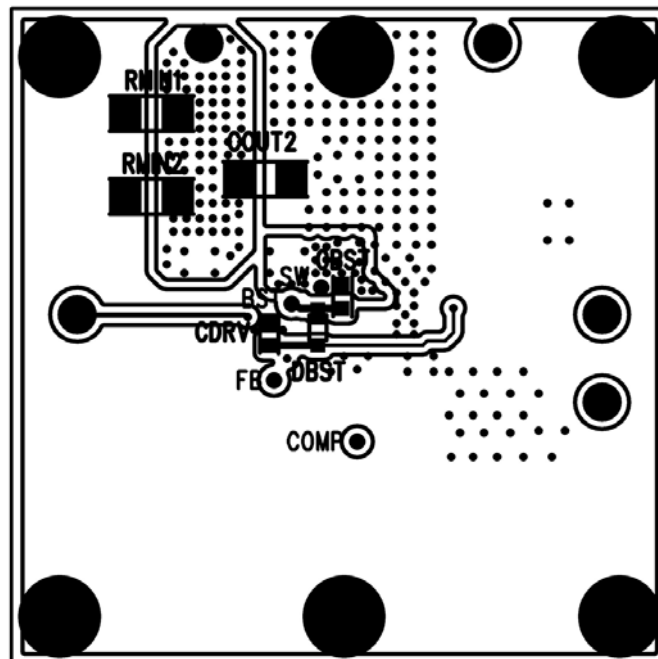
Figure 17. Bottom View
