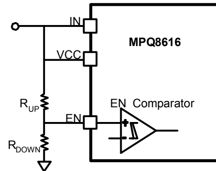
Figure 6—Adjustable UVLO
