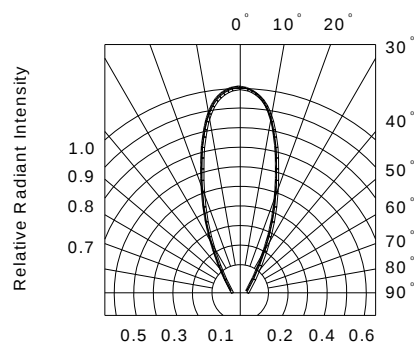
FIG.6 RADIATION DIAGRAM
