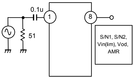
Test Circuit 1 S/N1, S/N2, Vin(lim), Vod, AMR
