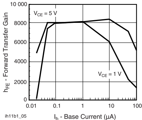
Fig. 5 - Non-Saturated and Saturated h FE vs. Base Current
