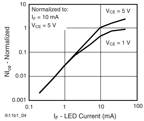
Fig. 4 - Normalized Non-Saturated and Saturated Collector Emitter Current vs. LED Current
