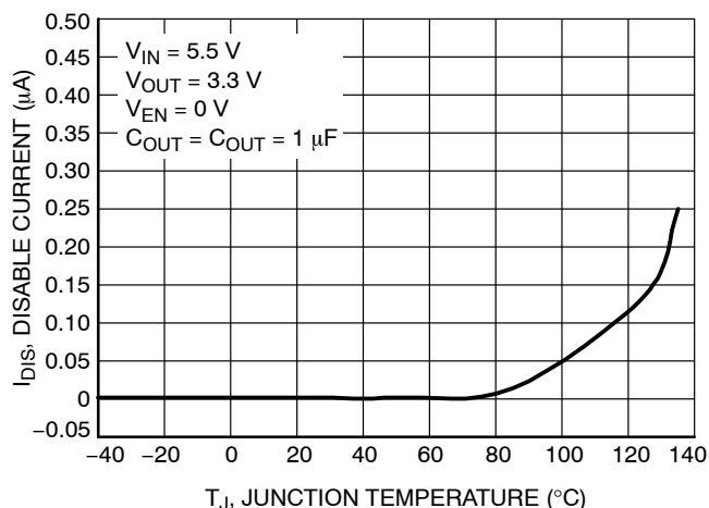
Figure 30. Disable Current vs. Temperature, V_{OUT} = 3.3\text{ V}
