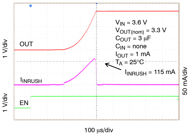
Figure 37. Enable Turn-On Response, V_{OUT} = 3.3 V, C_{OUT} = 3 μF
