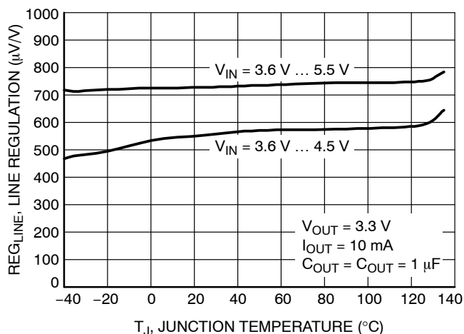
Figure 28. Line Regulation vs. Temperature, V_{OUT} = 3.3\text{ V}
