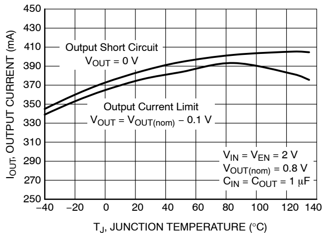
Figure 32. Output Current Limit vs. Temperature, V_{OUT} = 0.8\text{ V}
