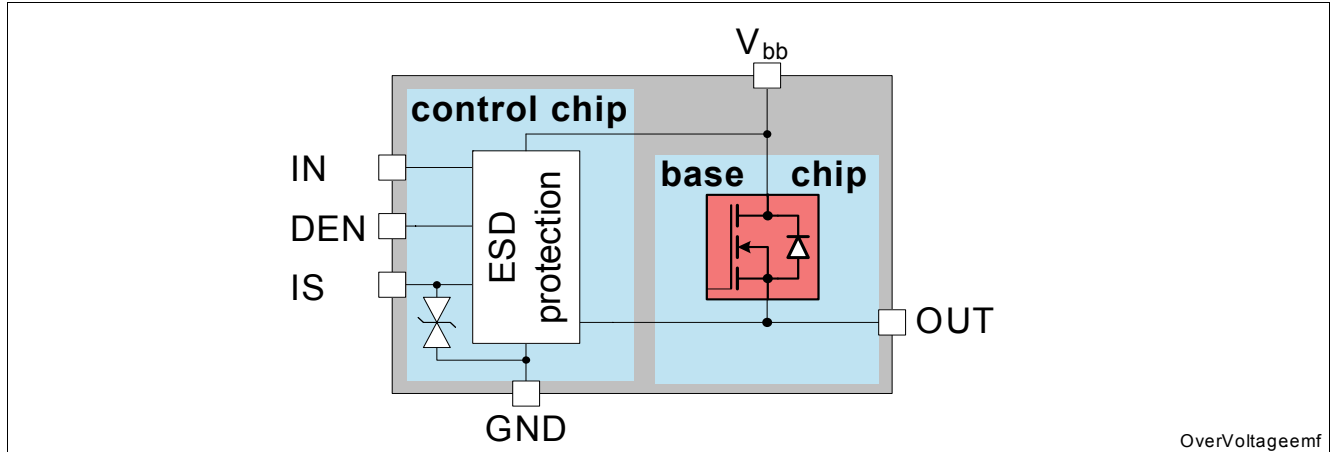
Figure 18 Over-Voltage Protection
