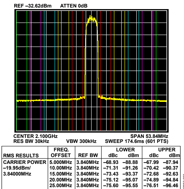
Figure 55. One-Carrier WCDMA ACLR in Mix Mode, f_{OUT} = 2.1 GHz, f_{DAC} = 2304 MHz, Full-Scale Current = 20 mA
