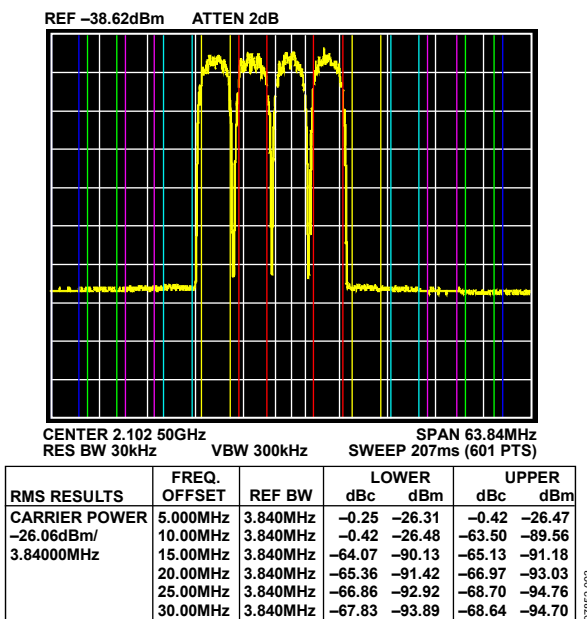
Figure 56. Four-Carrier WCDMA ACLR in Mix Mode, f_{OUT} = 2.1 GHz, f_{DAC} = 2304 MHz, Full-Scale Current = 20 mA
