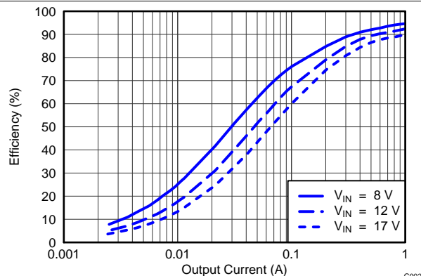
Figure 43. Efficiency vs Output Current
