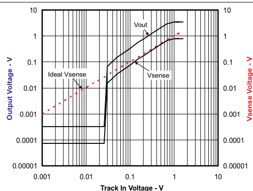
Figure 40. Tracking Performance
