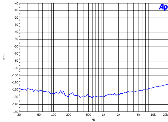
Figure 11. 48 kHz, Crosstalk
