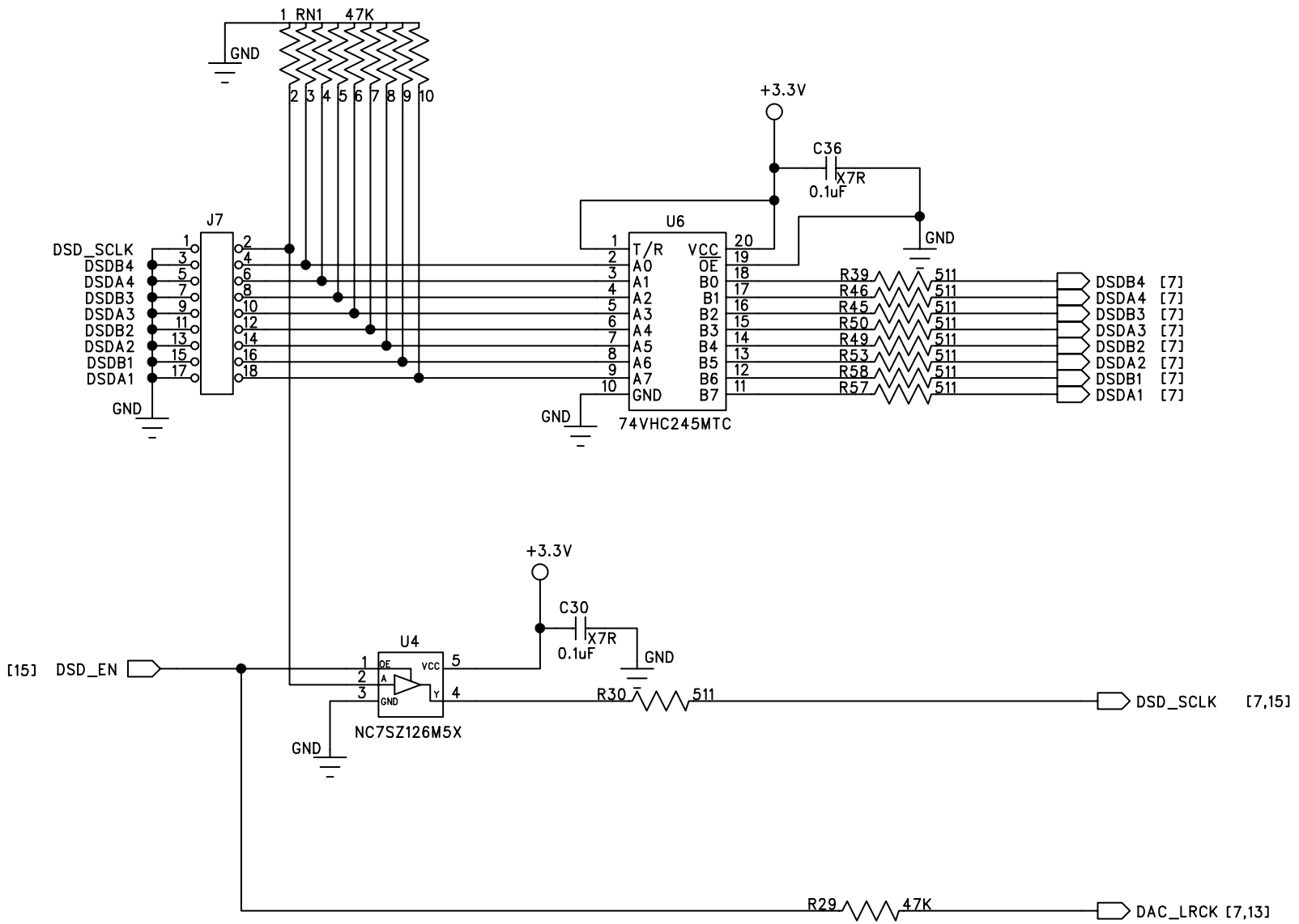
Figure 50. DSD Input Header
