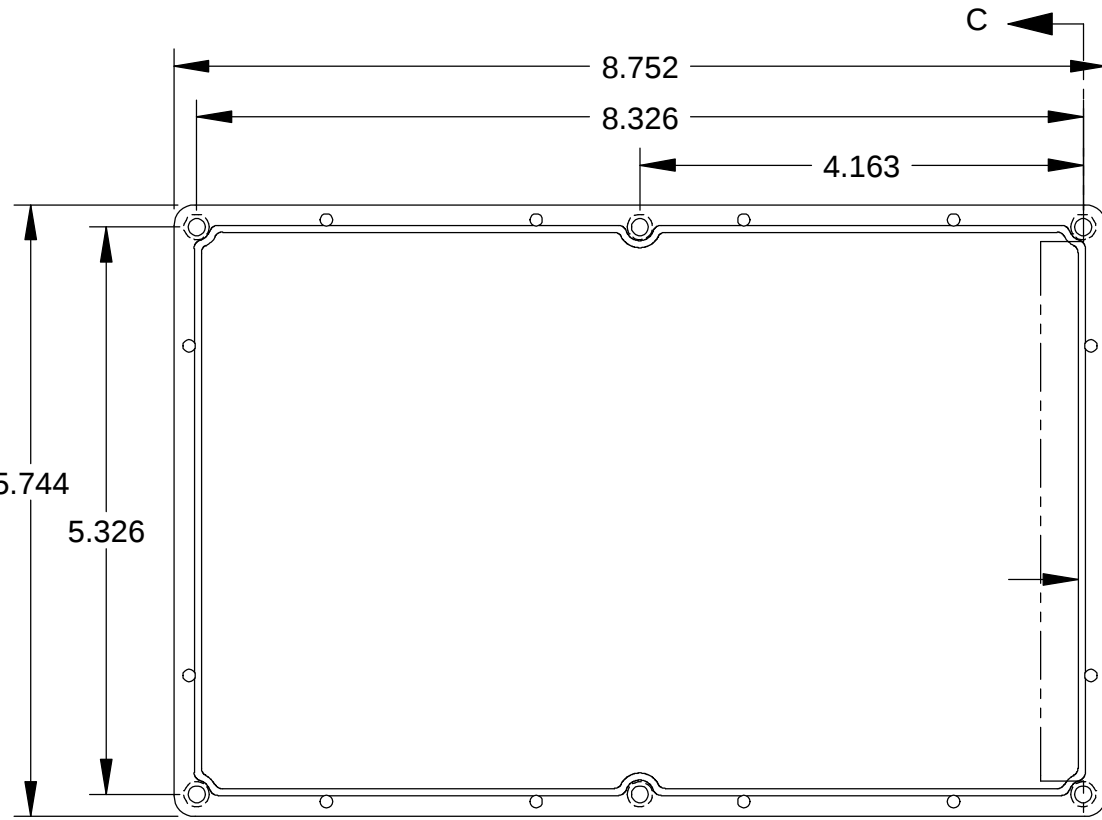
SECTION C-C
