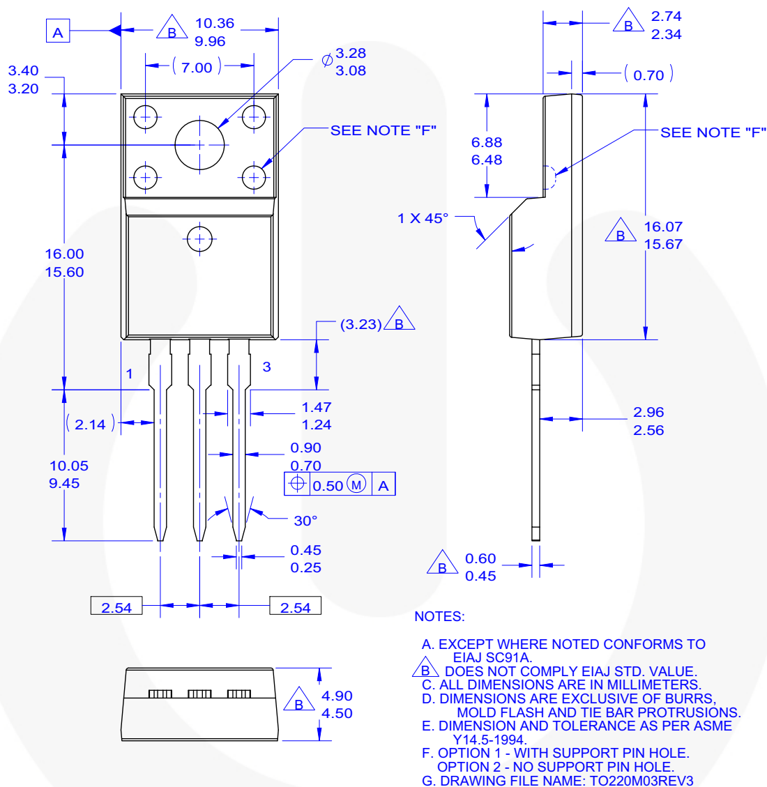
Figure 9. TO220, MOLDED, 3-LEAD, FULL PACK, EIAJ SC91, STRAIGHT LEAD
