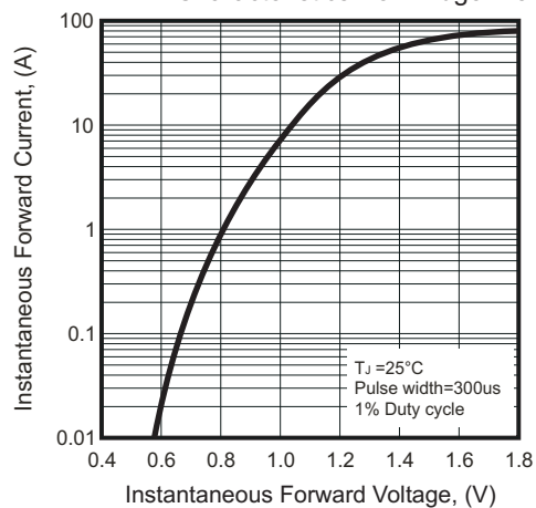
Fig.2 - Typical Instantaneous Forward Characteristics Per Bridge Element
