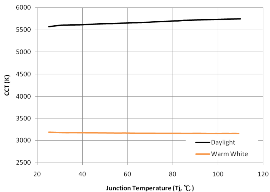
Fig.13 CCT vs junction temperature - White
