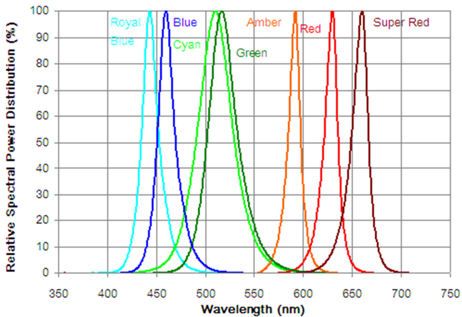
Fig.2 Normalised spectral power distribution – Royal Blue, Blue, Cyan, Green, Amber, Red, Super Red
