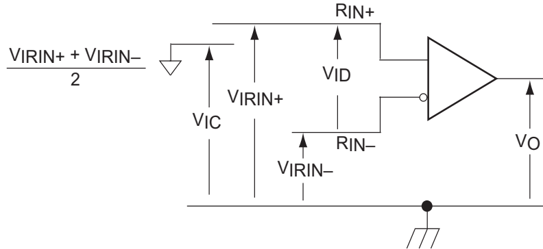
Figure 1. Voltage Definitions
