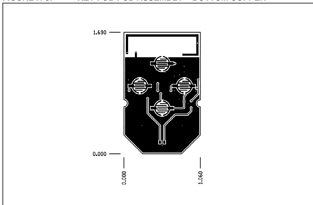
FIGURE A-3: KEY FOB PCB ASSEMBLY – BOTTOM COPPER
