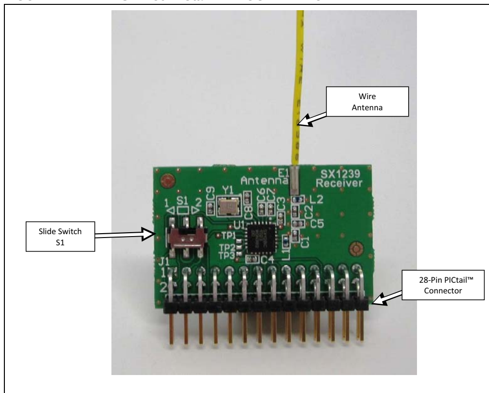
FIGURE 4-1: SX1239 PICtail™ DAUGHTER BOARD
