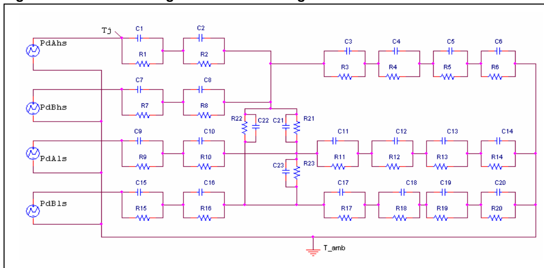
Figure 17. Thermal fitting model of an H-bridge in PowerSSO-36
