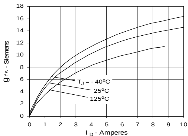
Fig. 9. Transconductance
