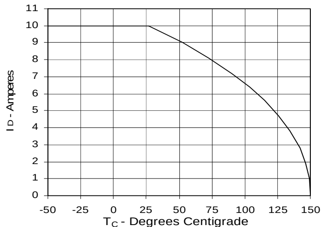
Fig. 7. Drain Current vs. Case Temperature
