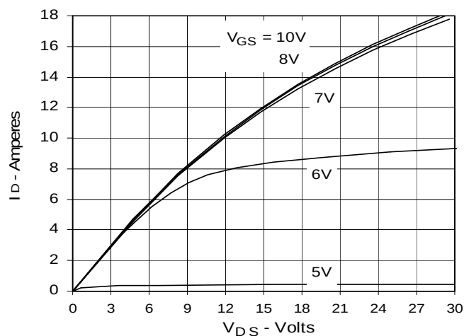
Fig. 3. Extended Output Characteristics @ 25°C
