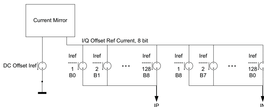
Figure 95. Block Diagram of the Programmable Current DAC
