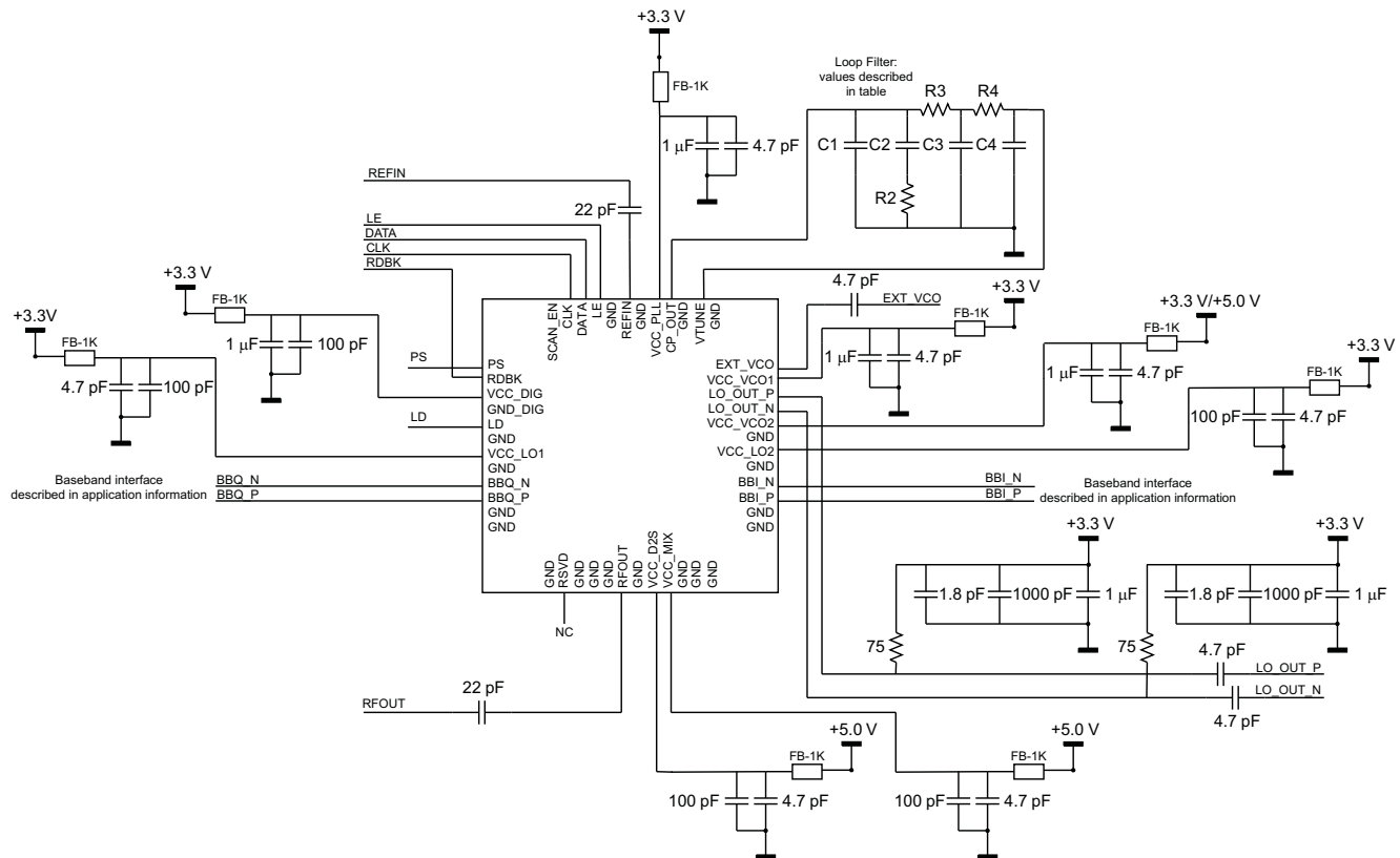
Figure 96. Application Schematic
