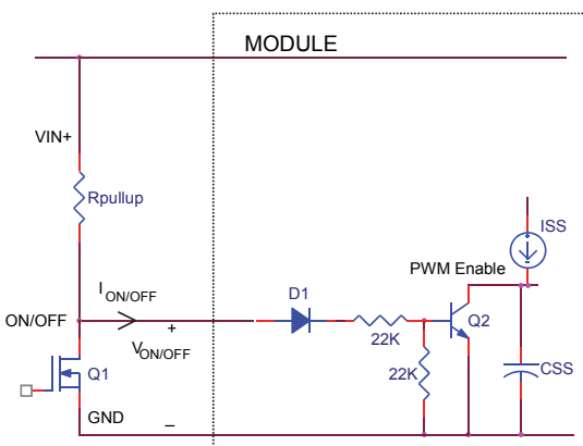
Figure 32. Circuit configuration for using positive On/Off logic.
