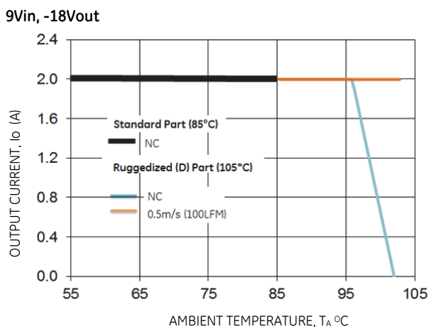
Figure 61. Derating Output Current versus Ambient Temperature and Airflow.
