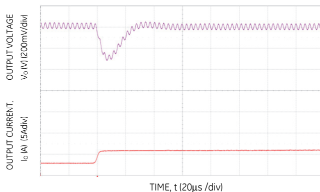
Figure 22. Transient Response to Dynamic Load Change from 50% to 100% at 28V in , C ext = 5x22μF, C Tune = 220pF & R Tune = 200
