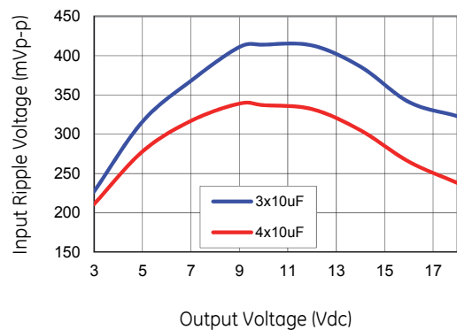
Figure 29. Input ripple voltage for various output voltages with 3x10 μF or 4x10 μF ceramic capacitors at the input (maximum load). Input voltage is 28V. Scope BW at 20MHz
