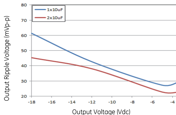
Figure 69. Output ripple with 1x10μF or 2x10μF output ceramic capacitors (max load).
