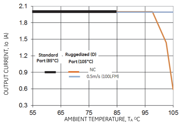
Figure 63. Derating Output Current versus Ambient Temperature and Airflow.
