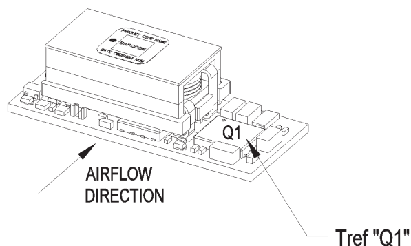
Figure 41. Preferred airflow direction and location of hot-spot of the module ( T_{ref} ).
