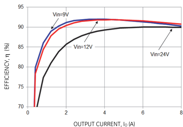
Figure 49. Converter Efficiency versus Output Current.
