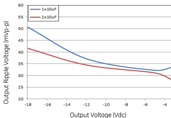
Figure 67. Output ripple with 1x10μF or 2x10μF output ceramic capacitors (max load).
