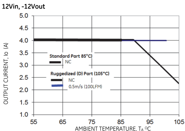
Figure 59. Derating Output Current versus Ambient Temperature and Airflow.
