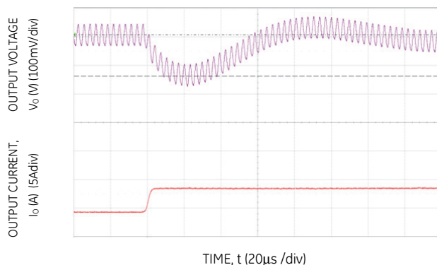
Figure 16. Transient Response to Dynamic Load Change from 50% to 100% at 28Vin, C ext – 1x22μF+1x470μF, C Tune =1.5nF & R Tune =200
