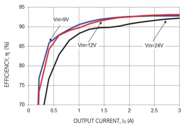
Figure 50. Converter Efficiency versus Output Current.
