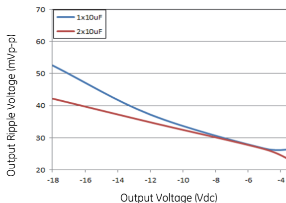
Figure 68. Output ripple with 1x10μF or 2x10μF output ceramic capacitors (max load).
