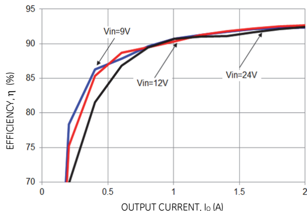
Figure 51. Converter Efficiency versus Output Current.
