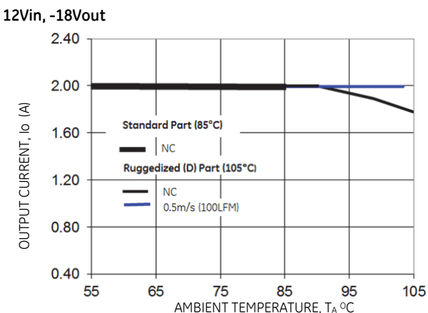
Figure 62. Derating Output Current versus Ambient Temperature and Airflow.
