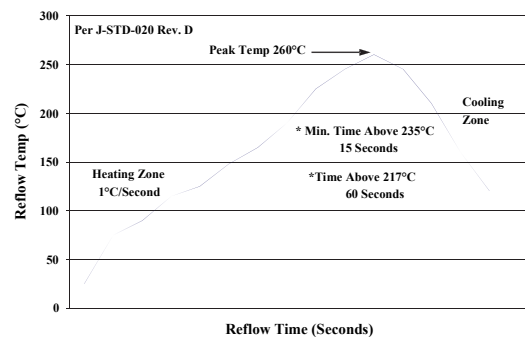
Figure 42. Recommended linear reflow profile using Sn/Ag/Cu solder.
