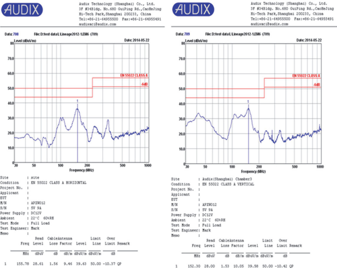
Fig 43 – EMI Plot of APXW012 on evaluation board with 12 V in, 5Vo @ 9 A out
