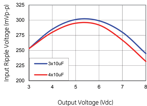
Figure 28. Input ripple voltage for various output voltages with 3x10 μF or 4x10 μF ceramic capacitors at the input (maximum load). Input voltage is 12V. Scope BW at 20MHz
