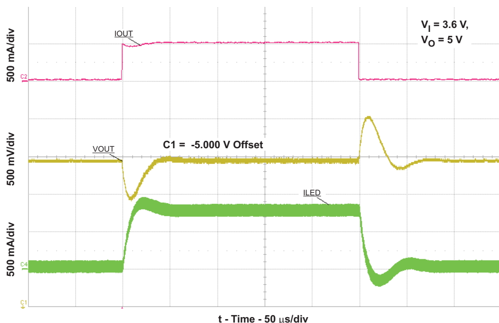
Figure 8. Voltage Mode Load Transient
