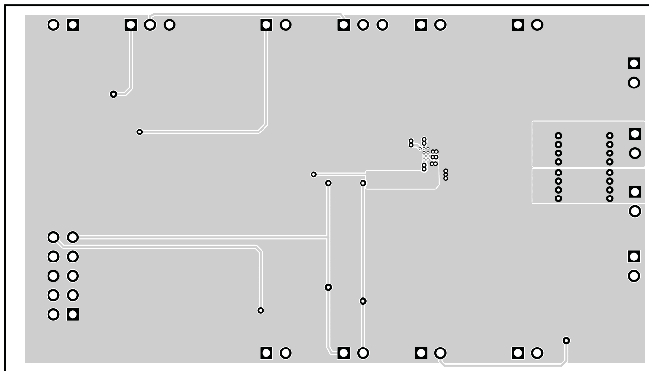
Figure 13. Bottom Layer
