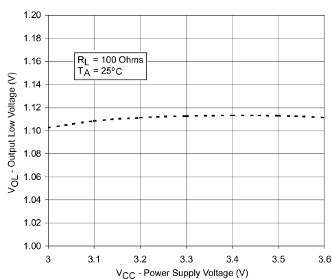
FIGURE 5. Output Low Voltage vs. Power Supply Voltage
