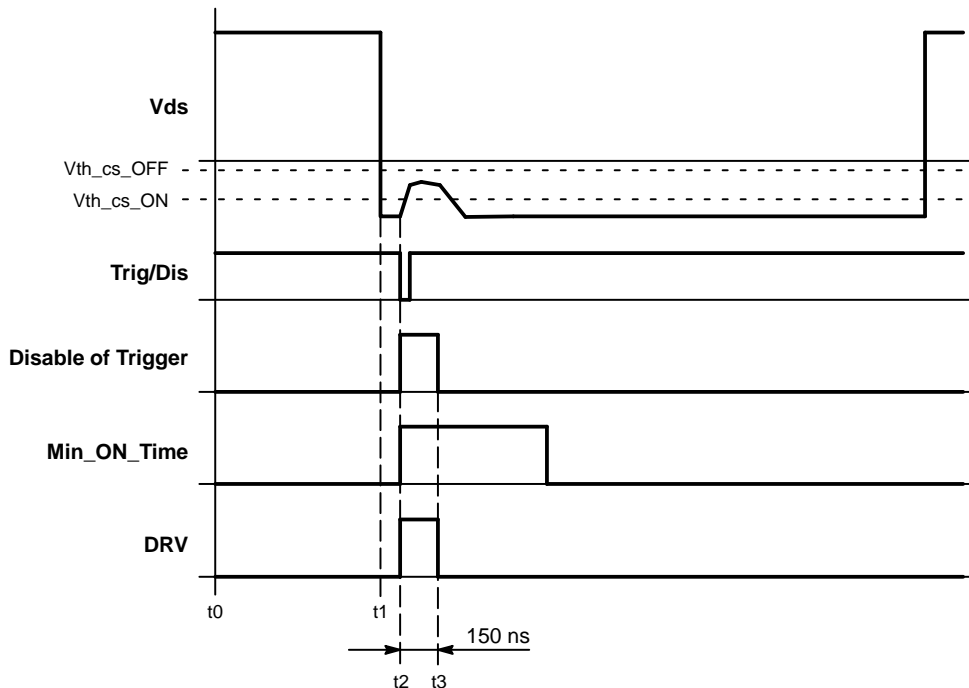
Figure 48. Trigger Needle Pulse and Trigger Blank Sequence
