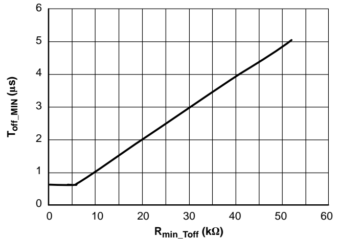
Figure 62. Min_Toff Adjust Characteristic
