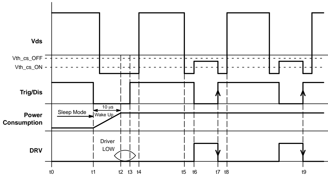
Figure 56. Waking-up Sequence
