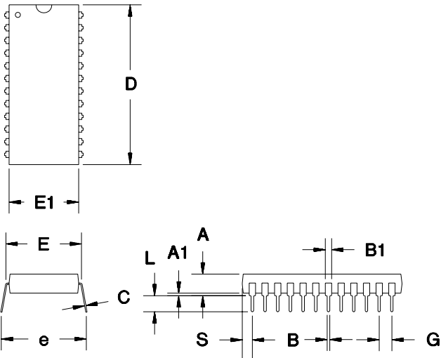
24-Pin DIP (0.600" DIP)
