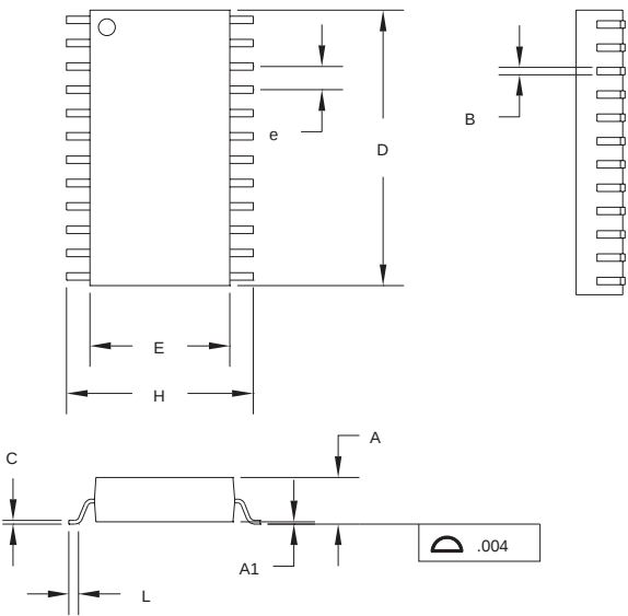
24-Pin S (0.300" SOIC)
