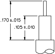
CABLE STRIP DIMENSIONS
