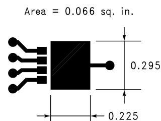
Figure 21. SCENARIO B, \theta_{JA} = 125^{\circ}\text{C/W}
