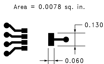
Figure 20. SCENARIO A, \theta_{JA} = 148^{\circ}\text{C/W}
