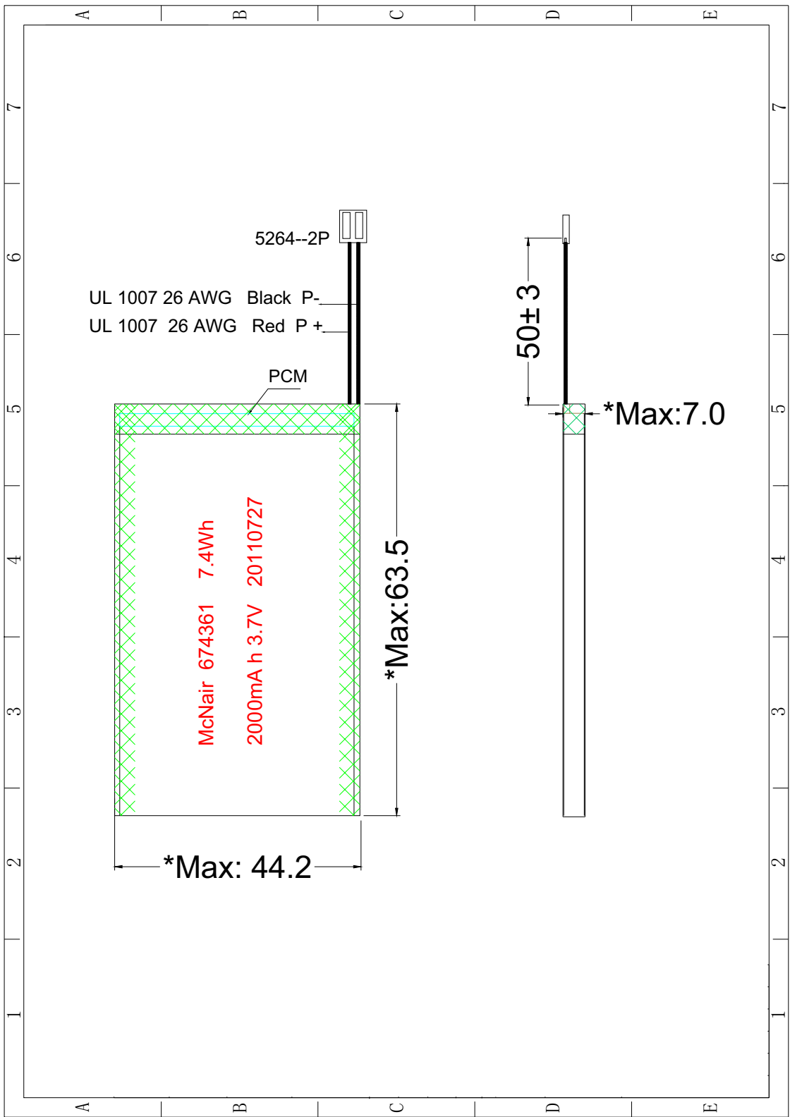
Fig.1 OUTLINE DRAWING
