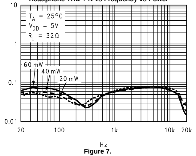
Headphone THD + N vs Frequency vs Power
