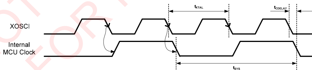
Figure 33 – Internal MCU Clock Timing
