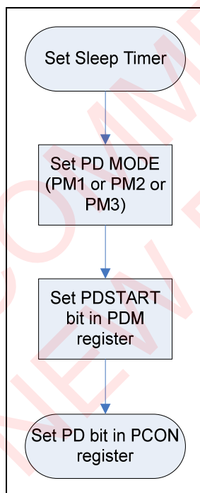
Figure 11 – Power-Down mode setting procedure
