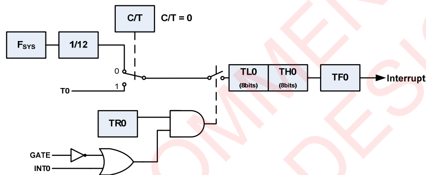
Figure 13 – Timer0 Mode1
