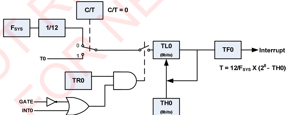
Figure 14 – Timer0 Mode2
