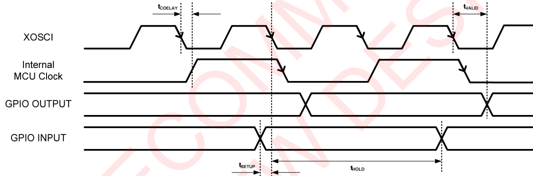
Figure 36 – GPIO Timing
