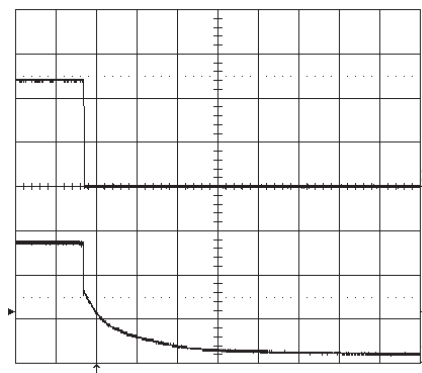
Turn-off at I_o=4.2 A resistive load at T_{Pcb}=+25 °C, V_{in}=27 V. Turn-off enabled by disconnecting V_{in} . Top trace: output voltage (10 V/div.). Bottom trace: input voltage (5 V/div.). Time scale: 10 ms/div.
