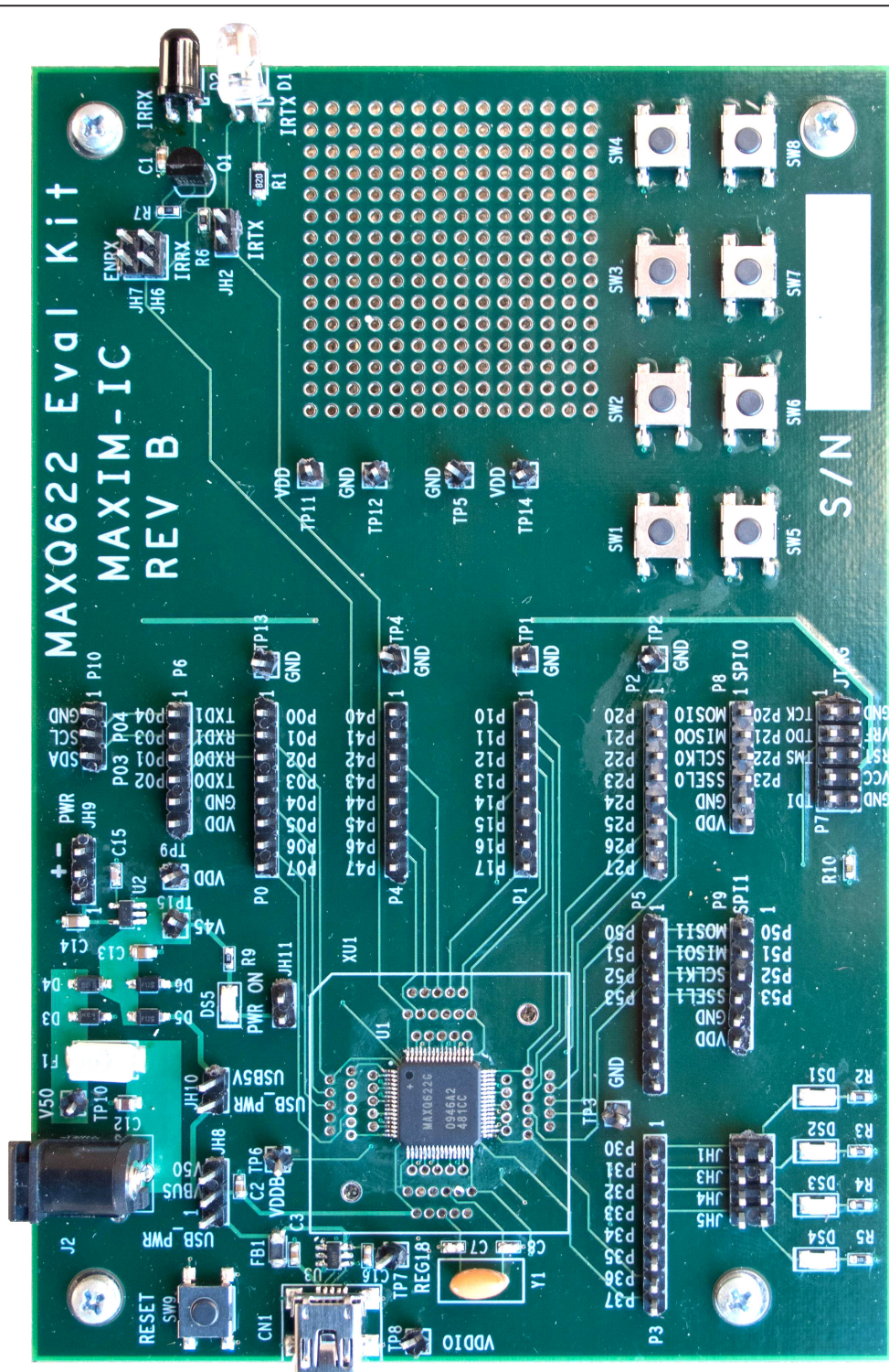
Figure 1. MAXQ622 EV Kit Board
