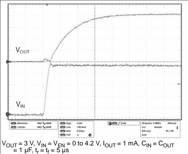
Figure 30. Startup transient
