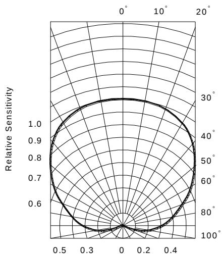
Fig.7 SENSITIVITY DIAGRAM
