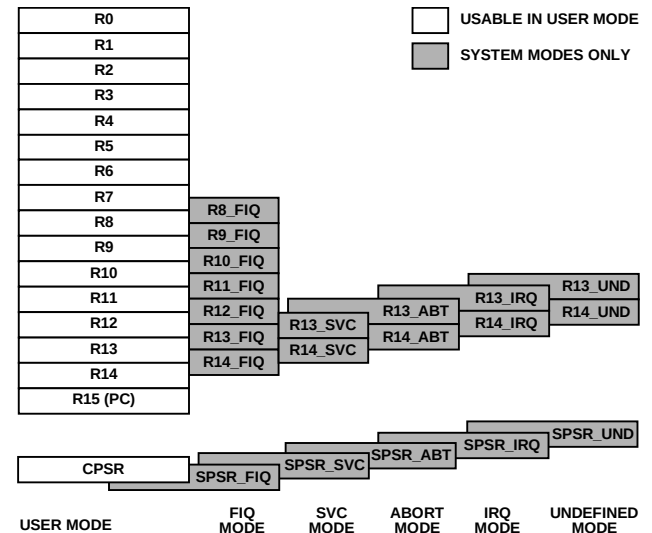
Figure 4. Register Organization
