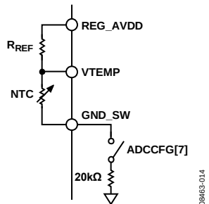
Figure 13. Internal Ground Switch Configuration
