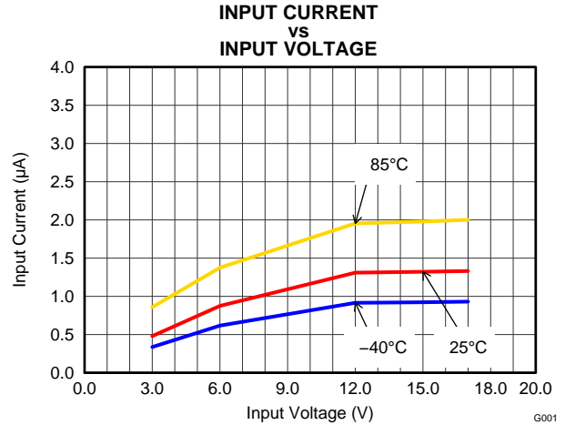
Figure 18. Shutdown Current
