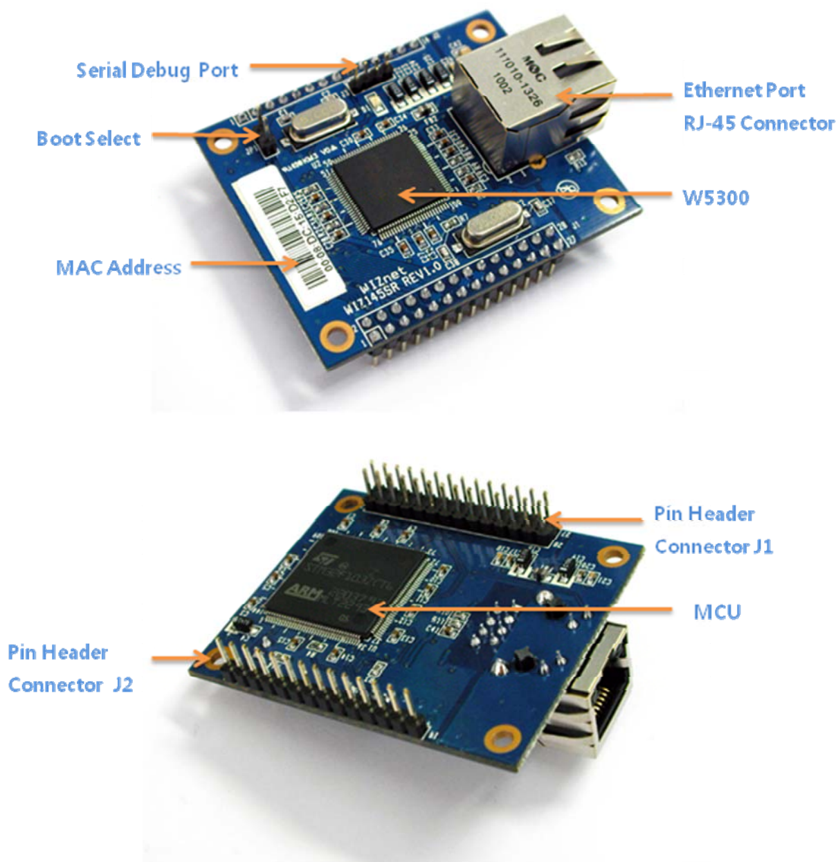
Figure 2. WIZ145SR Module Interface
