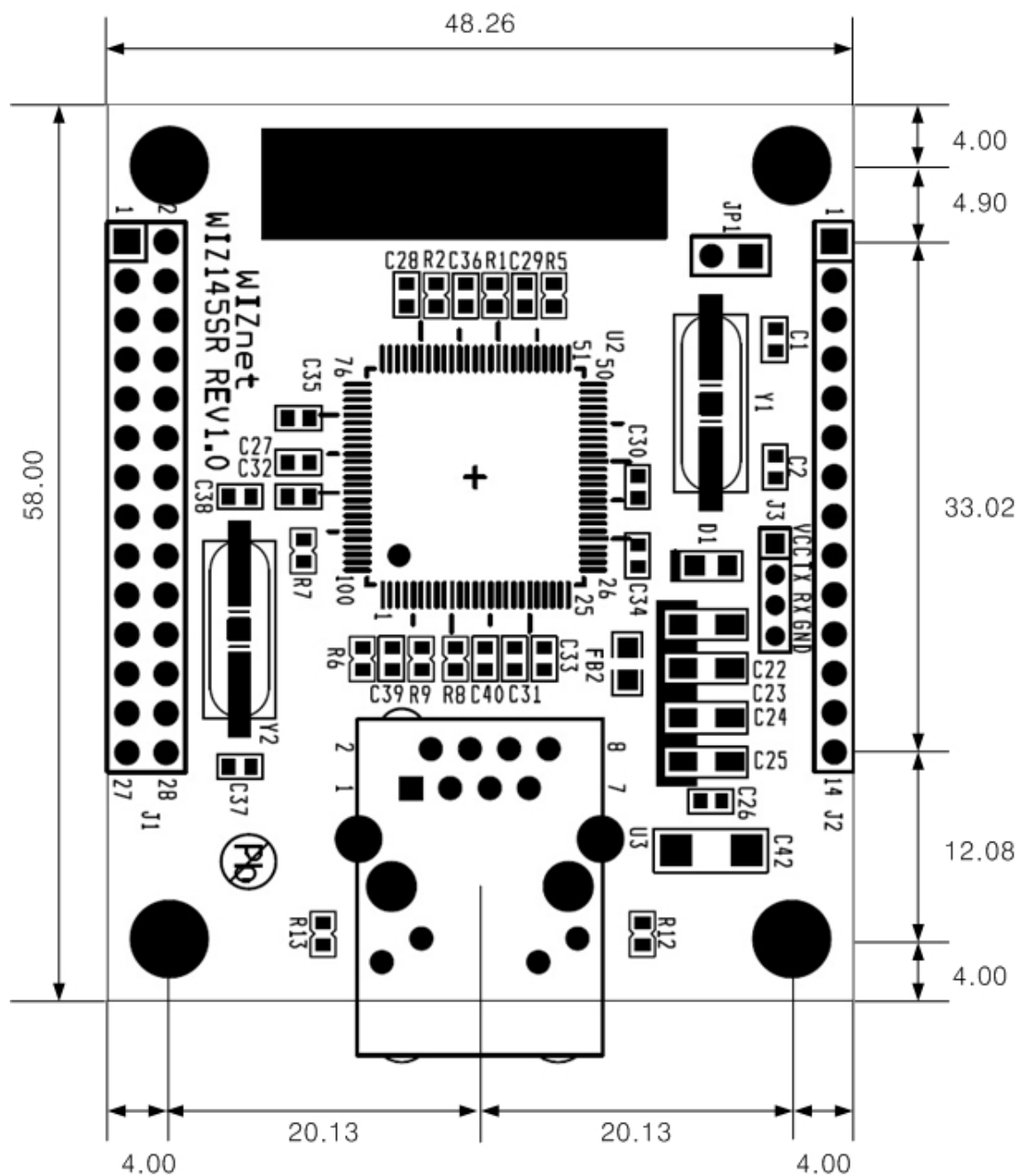
Figure 5. WIZ145SR Module Dimension (mm)
