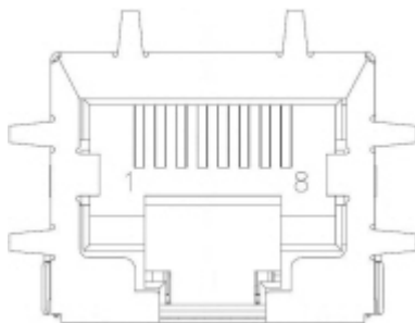
Figure 8. RJ-45 Connector
