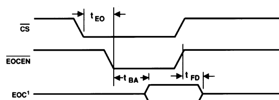
Figure 2. EOC Timing
