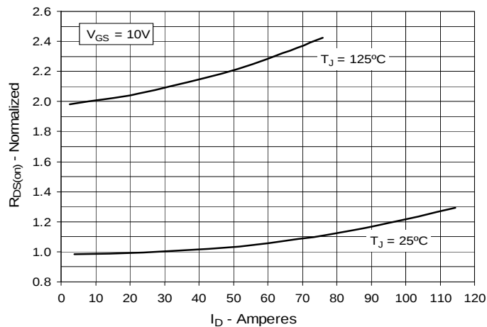
Fig. 5. R_{DS(on)} Normalized to I_D = 28A Value vs. Drain Current
