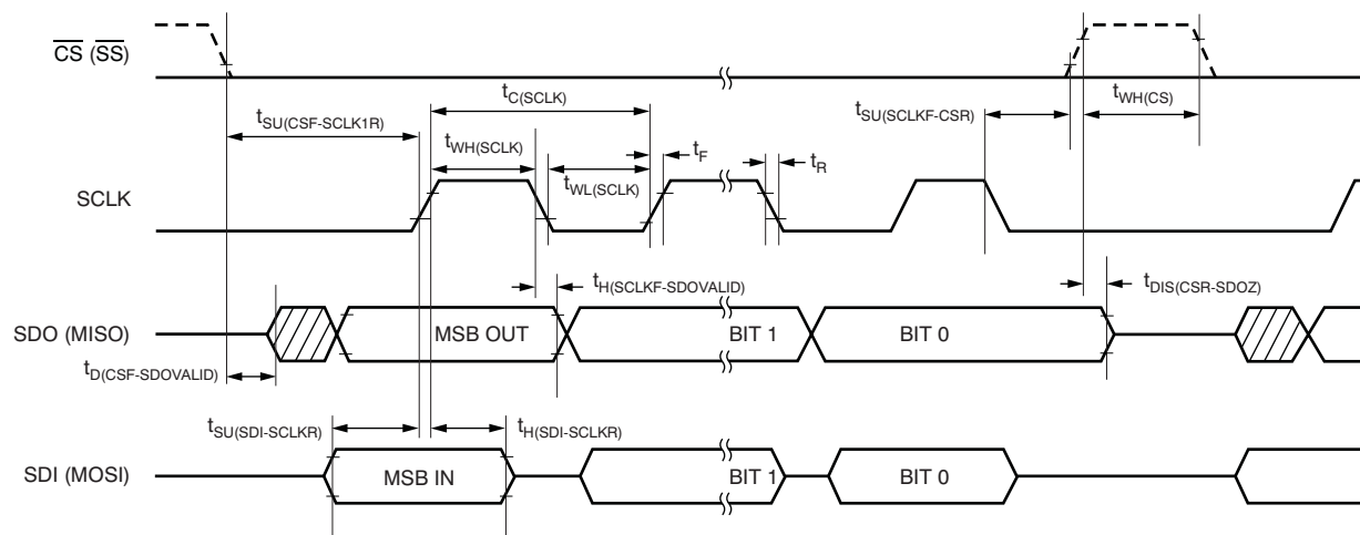
Figure 1. Detailed I/O Timing
