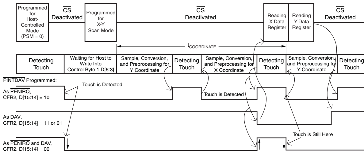
Figure 34. Example of an X and Y Coordinate Touch Screen Scan using TSMode 2
