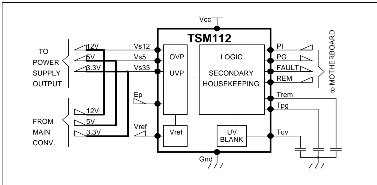
Figure 2 : Internal Schematic
