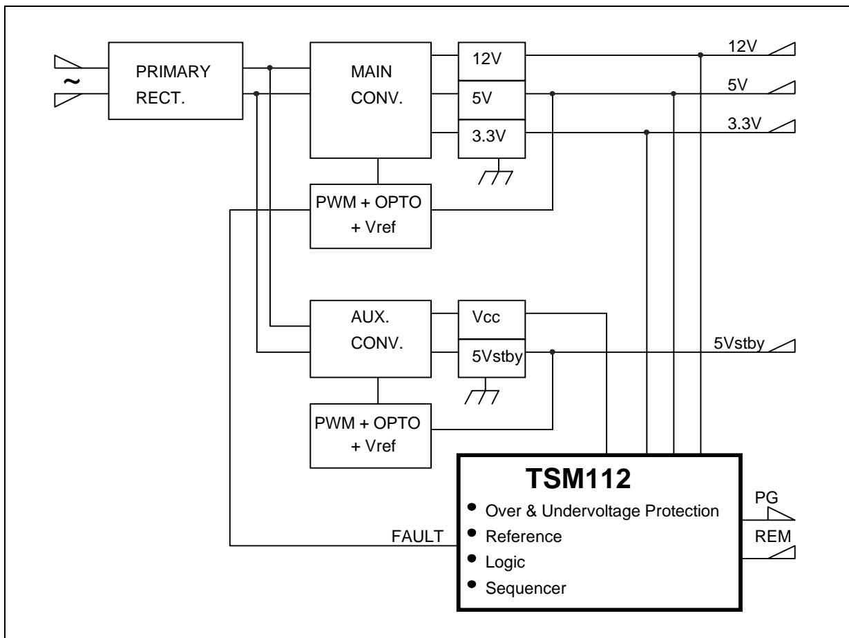
Figure 2 : Internal Schematic
