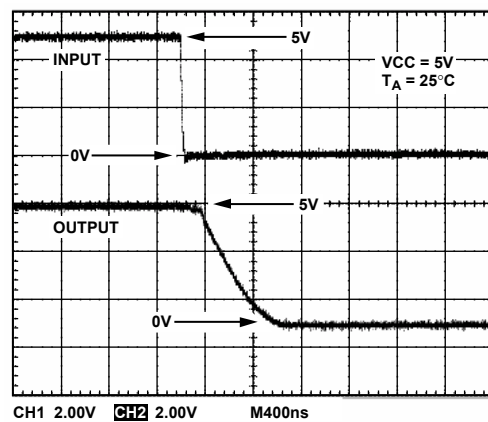
Figure 11. Transient Response—Falling
