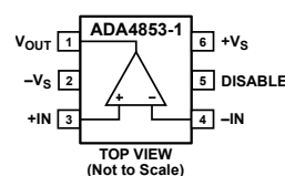
Figure 1. 6-Lead SC70
