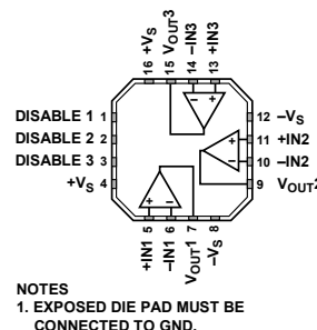
Figure 3. 16-Lead LFCSP_WQ
