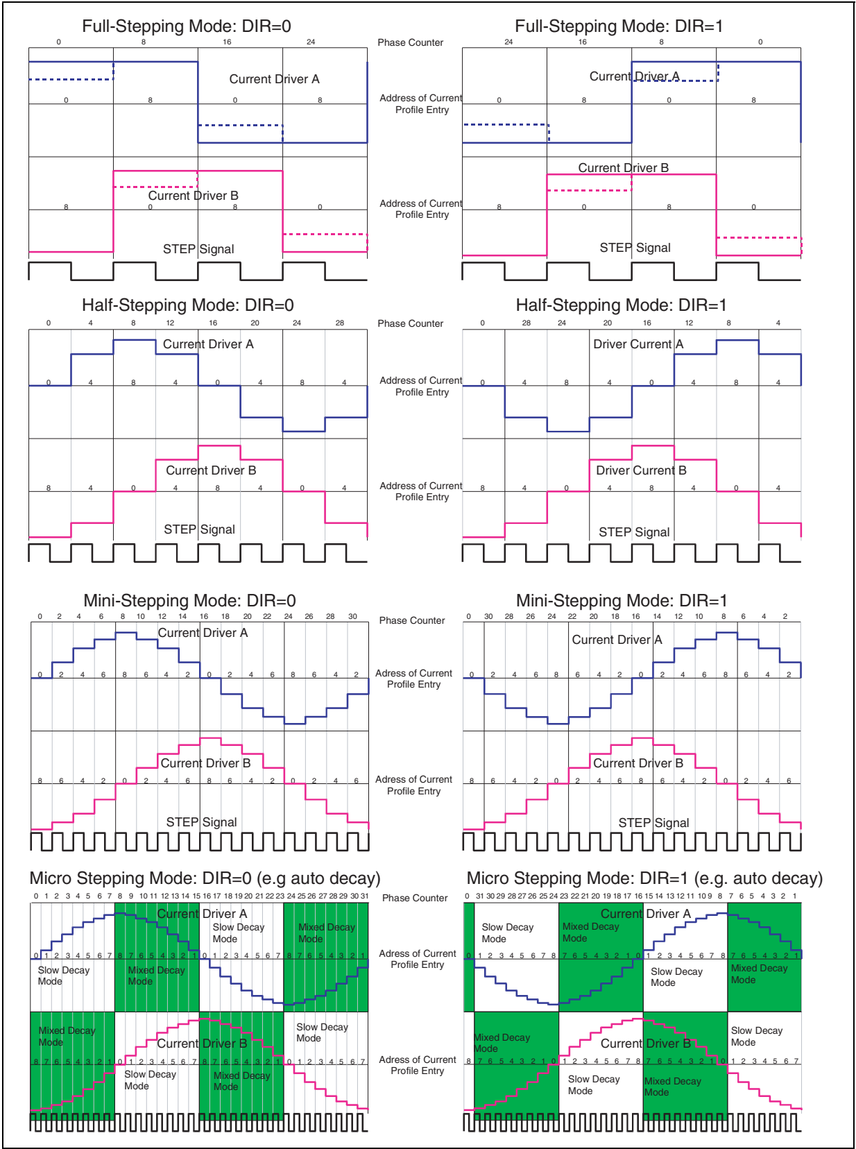
Figure 3. Stepping modes
