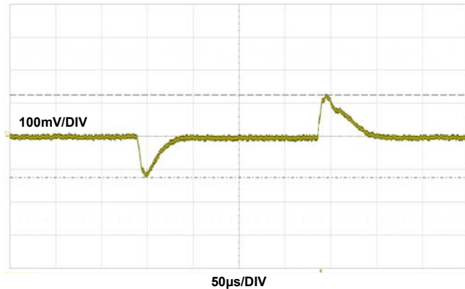
FIGURE 17. 0.9V OUT FOUR PHASE SINGLE OUTPUT TRANSIENT RESPONSE, I_{OUT} = 0A TO 40A , f_{SW} = 350kHz , C_{OUT} = 6 \times 330\mu F POSCAP+ 7 \times 47\mu F + 4 \times 100\mu F CERAMIC CAPACITOR
