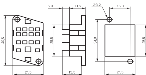
Chassis cut-out
