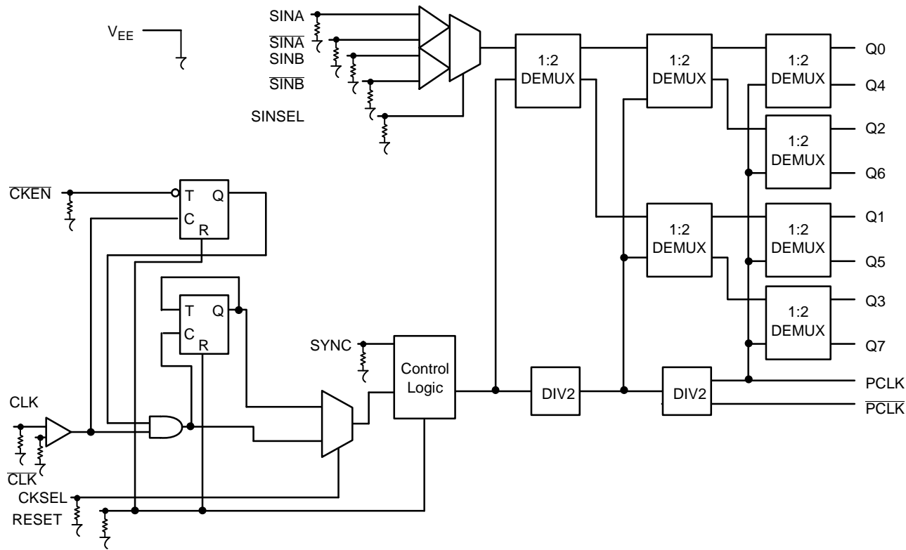
Figure 3. Logic Diagram
