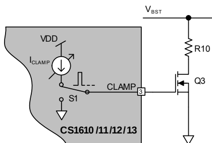
Figure 11. CLAMP Pin Model
